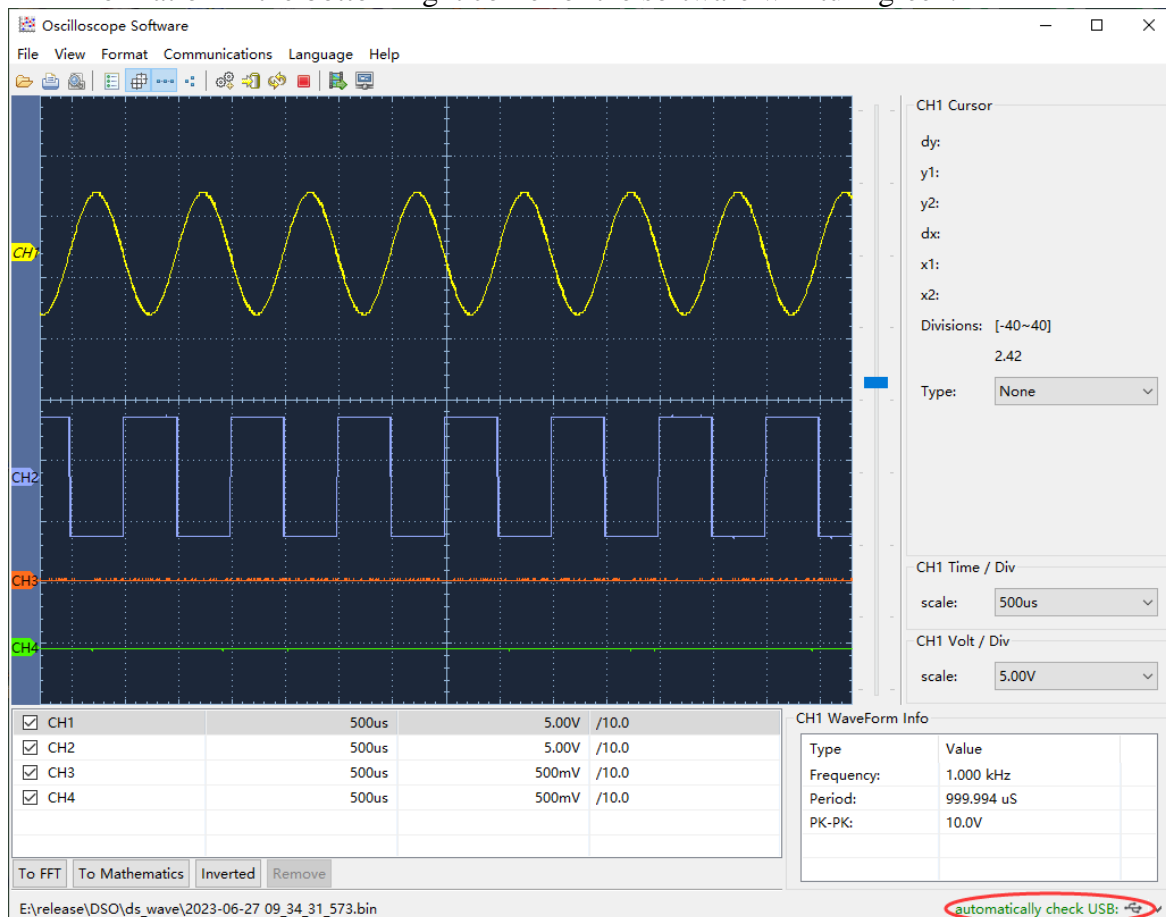
Figure 6-1 Connect with PC through USB port
