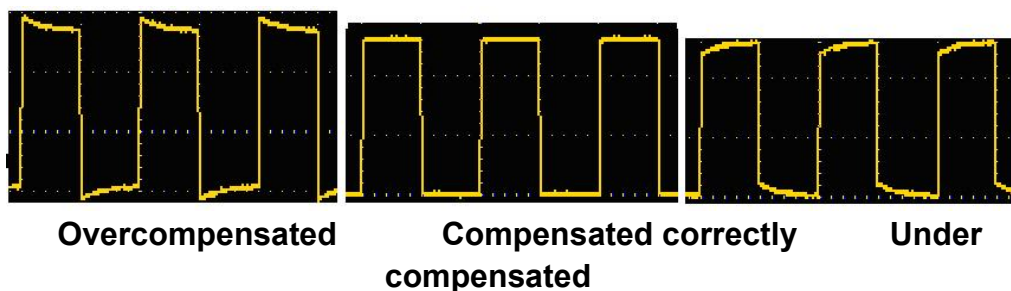
Figure 3-6 Displayed Waveforms of the Probe Compensation
