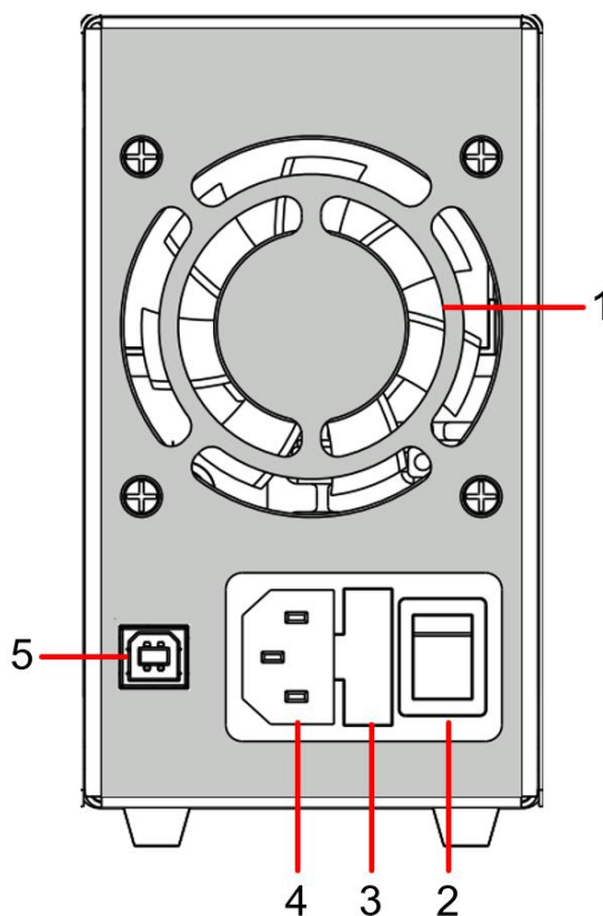
Figure 3- 2 Rear Panel Overview(Without USB model)
