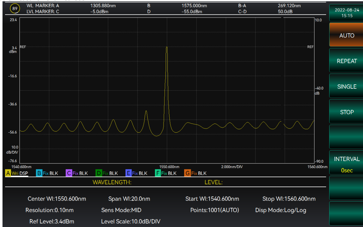
Figure 3-12 Auto-sweep end
