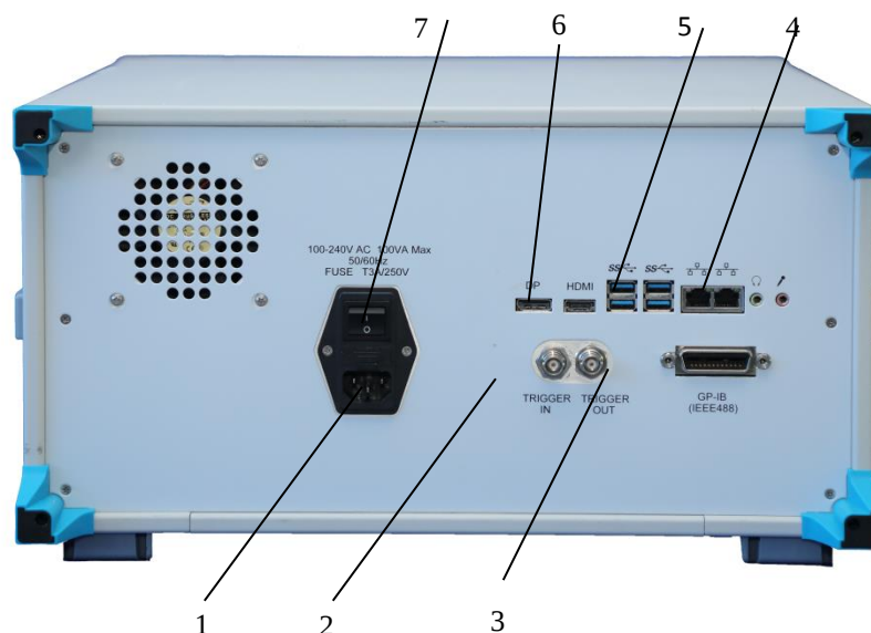
Figure 3-7 Rear panel of S6362D optical spectrum analyzer
