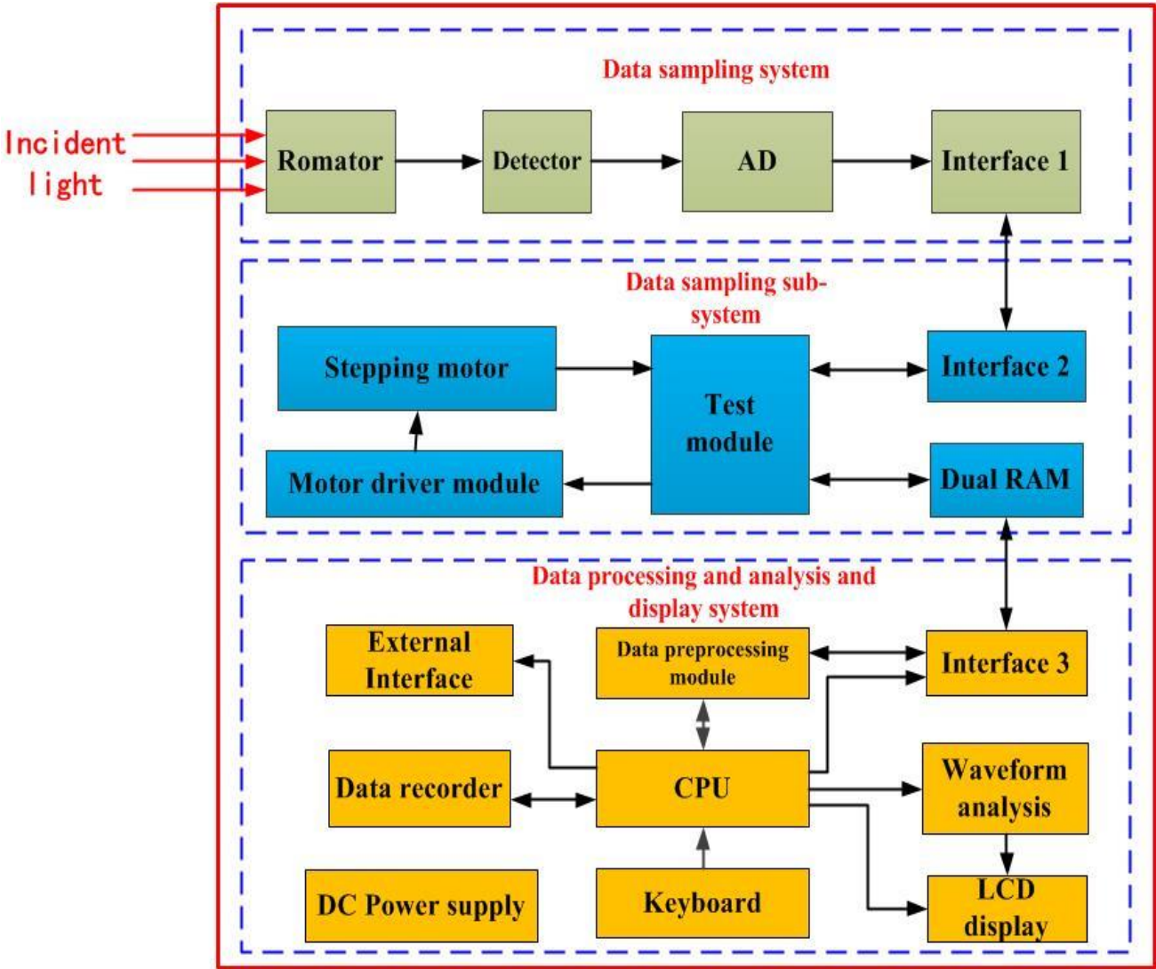
Figure 4-1 Block diagram of overall analyzer scheme
