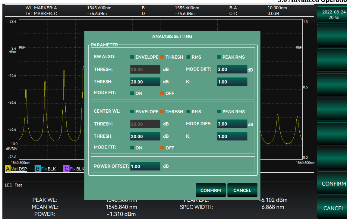
Figure 3-62 Schematic diagram of LED test interface
