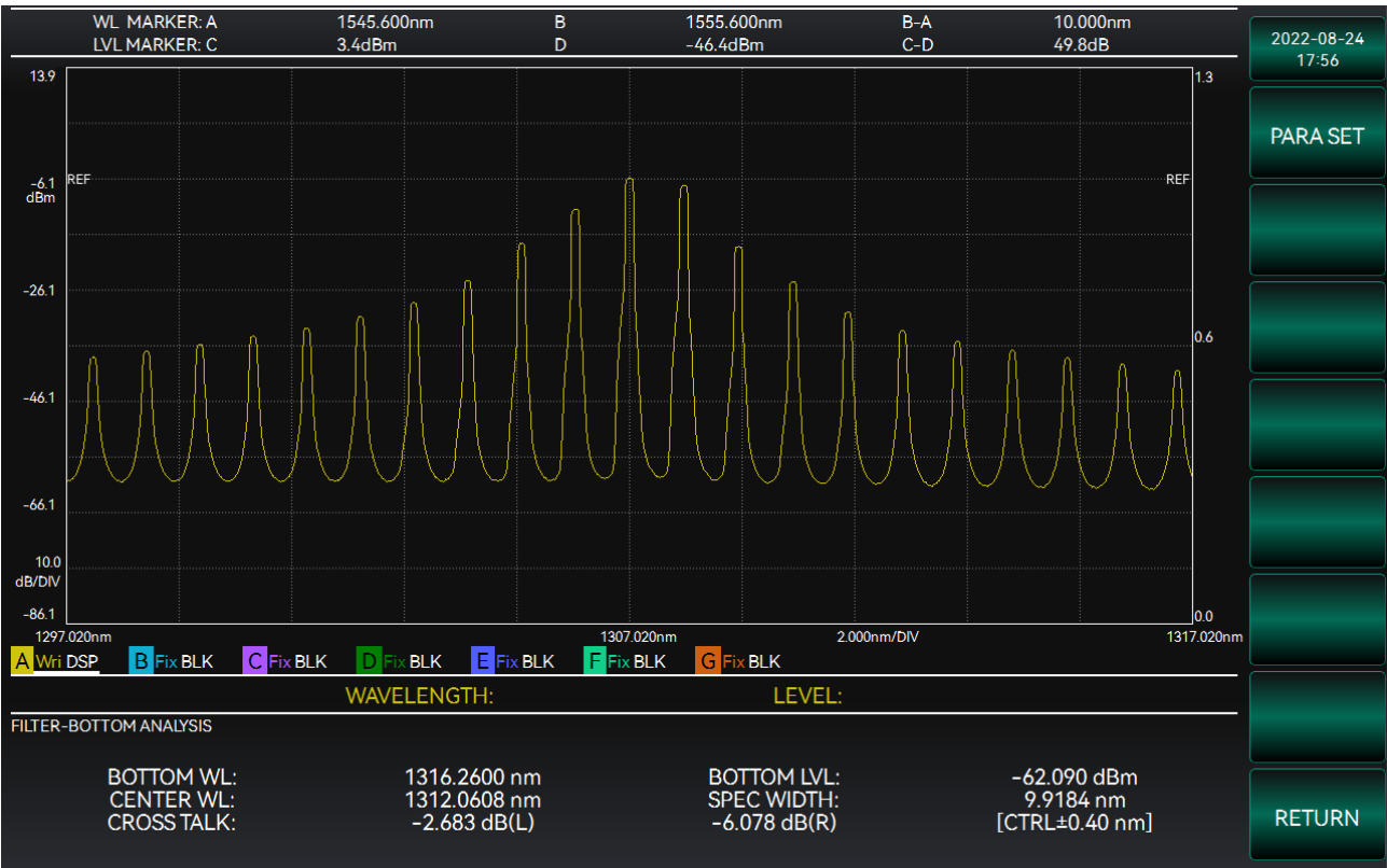
FILTER BOTTOM
