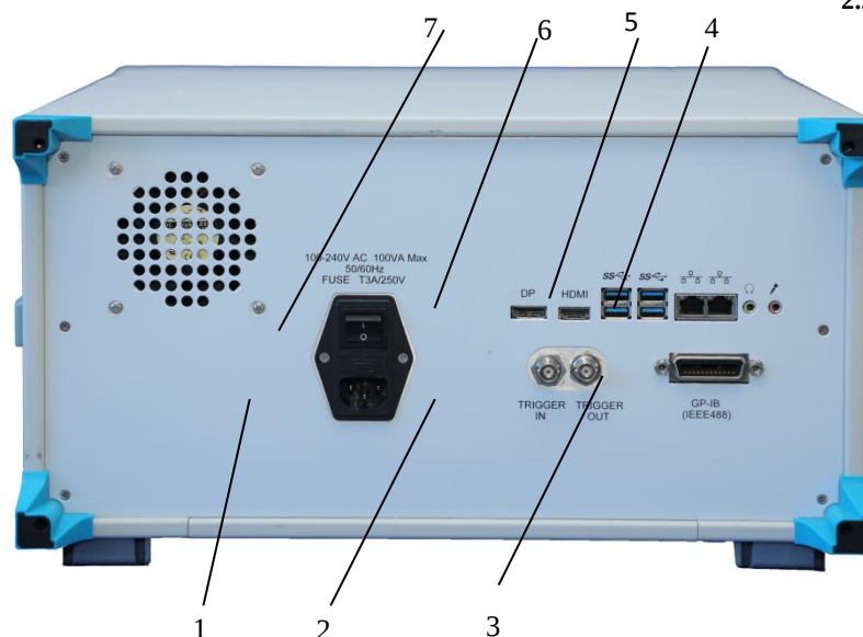
Figure 2-2 Rear panel interface of S6362D optical spectrum
