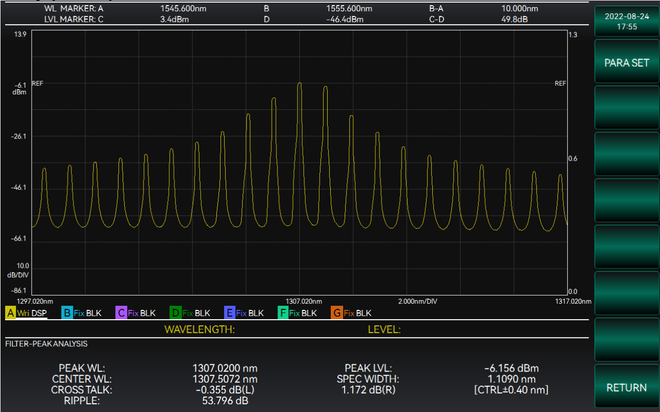
FILTER PEAK
